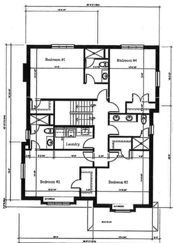
SECOND FLOOR PLAN — DETACHED HOUSE
