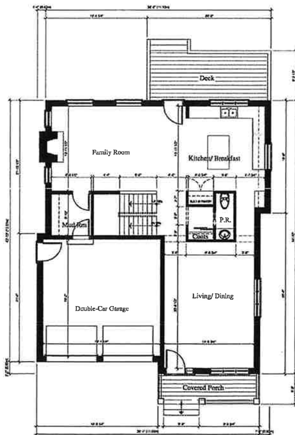
GROUND FLOOR PLAN — DETACHED HOUSE
