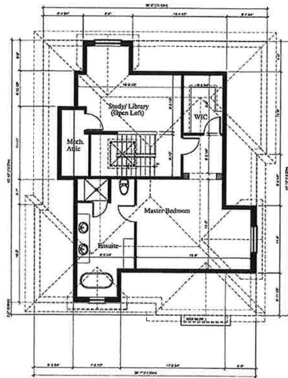
THIRD FLOOR PLAN — DETACHED HOUSE
